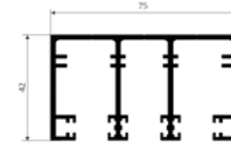
CARRIL SUPERIOR Top track
